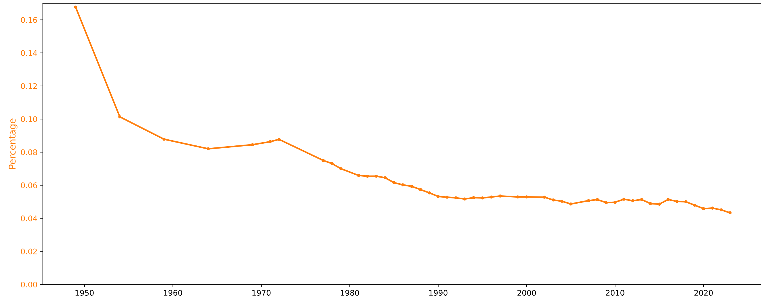
Japan ratio between population born(in 1 year) and (21 - 46) Women Population
